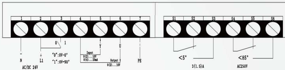
ExS6061Pro-SF On/Off
